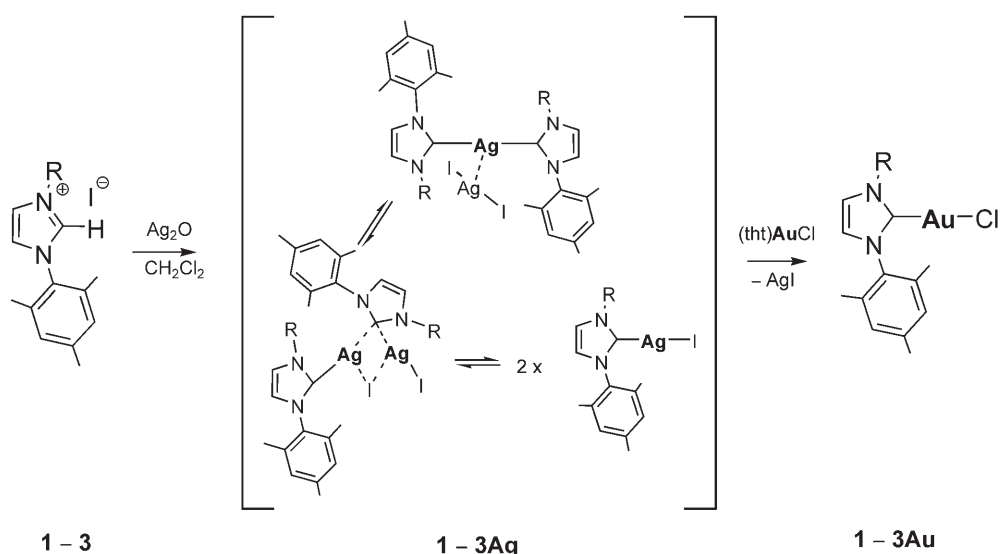
Scheme 2. Synthesis of gold-carbene complexes.
