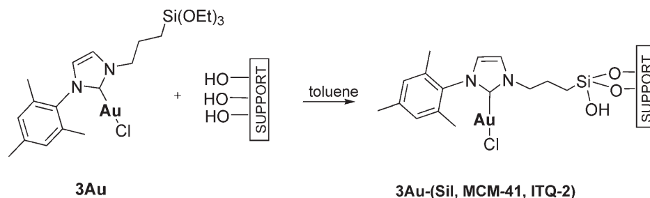
Scheme 3. Heterogenization of 3Au complex on silica, MCM-41 and ITQ-2.
