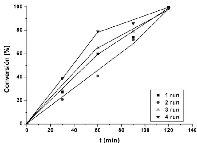
Figure 3. Recycling of 3Au-(MCM-41) in the hydrogenation of diethyl citraconate
