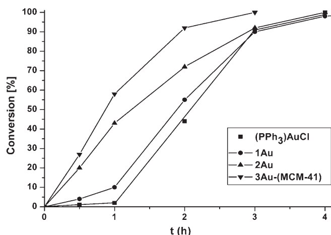
Figure 2. Comparison of the catalytic activities (homogeneous and heterogenized complexes) on the hydrogenation reaction of diethyl citraconate.
