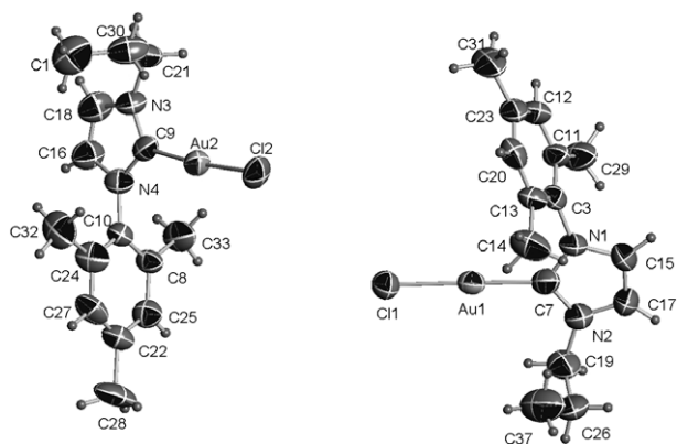
Figure 1. ORTEP representation for 2Au .
