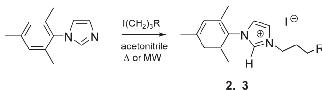
Scheme 1. Synthesis of imidazolium salts 2 and 3 .
